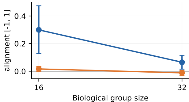
Escape alignment
